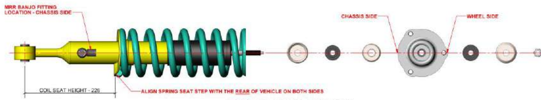
TOYOTA HILUX (2005-ON) RIGHT HAND STRUT SHOWN
